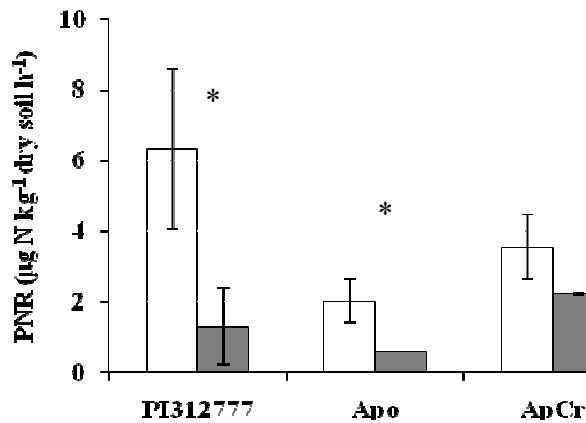
Fig. 3. Potential nitrification rates in the rhizosphere of three rice varieties (PI312777, Apo and ApCr) grown under two irrigation treatments, AC (white bars) and CF (grey bars). Vertical error bars represent the standard deviation; n = 3 .
