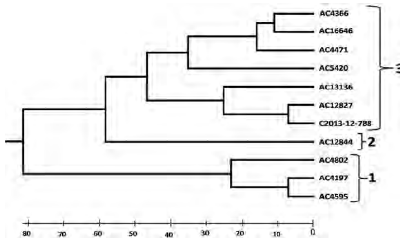
Fig. 3. Phylogenetic tree
